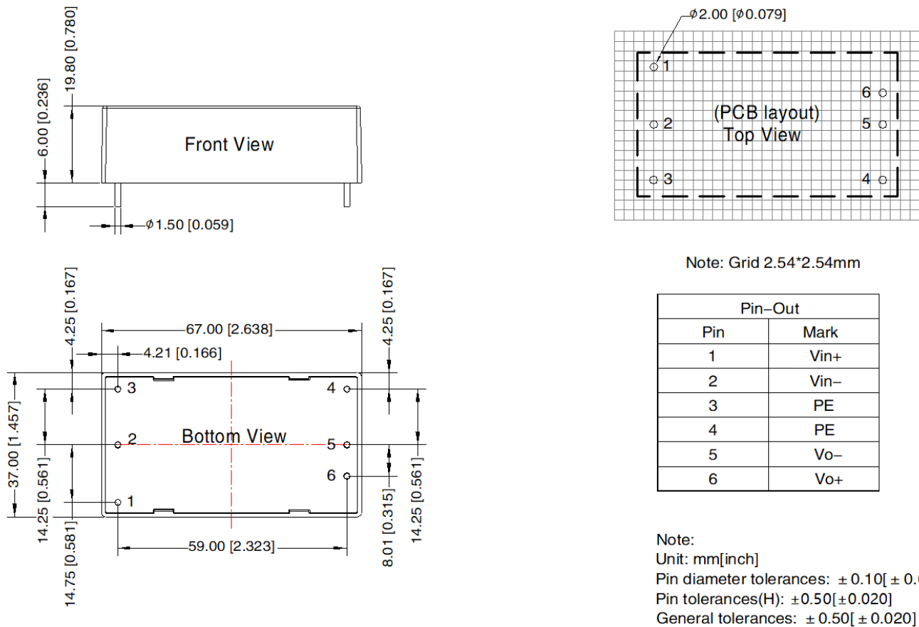
Figure 5. Mechanical drawing
