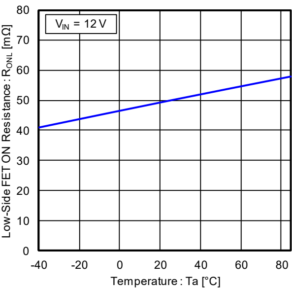
Figure 14. Low-Side FET ON Resistance vs Temperature
