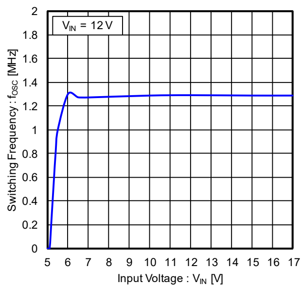
Figure 20. Switching Frequency vs Input Voltage ( V_{OUT} = 5.0\text{ V} , I_{OUT} = 1\text{ A} , \text{MODE} = \text{High} )
