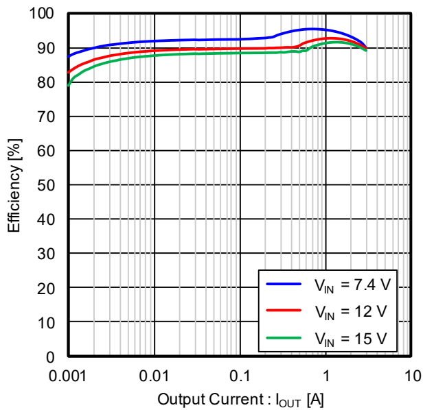
Figure 3. Efficiency vs Output Current (V OUT = 5 V, L = 2.2 μH, MODE = Low)
