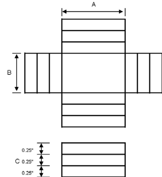
Each 0.025" section can be easily broken away to create shield heights of 0.25", 0.50" or 0.75"
