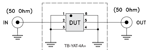
Fig 1. Block diagram of Test Circuit used for characterization, Test board TB-YAT-4A+ Conditions: Attenuation, VSWR: Pin=-10 dBm
