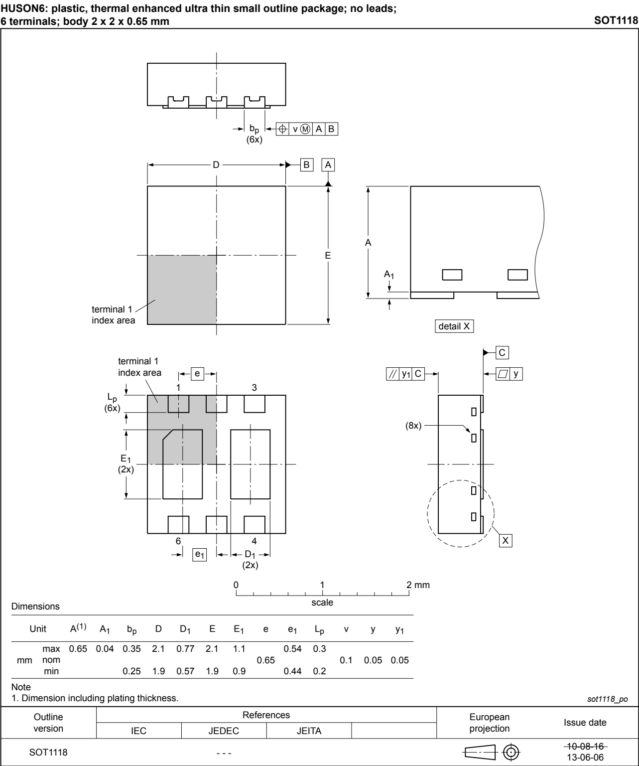
Fig. 18. Package outline DFN2020-6 (SOT1118)
