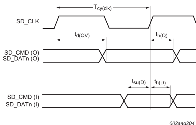
Fig 39. SD/MMC timing
