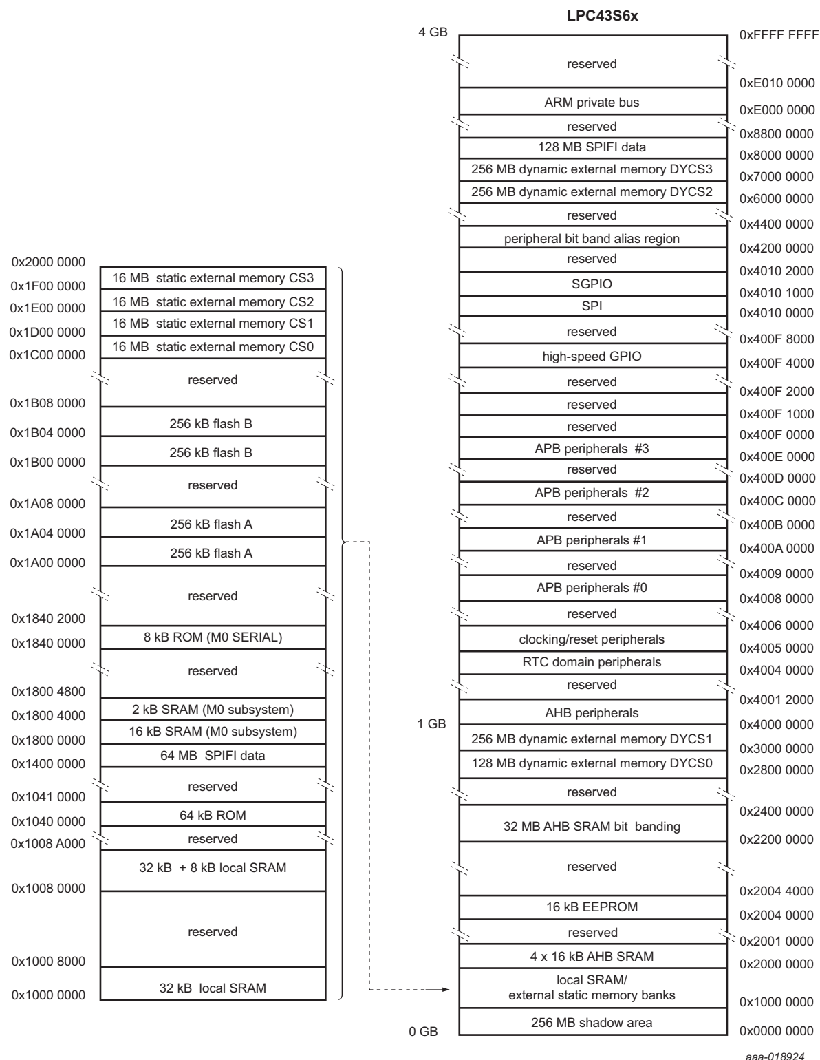
Fig 6. LPC43S6x Memory mapping (overview)
