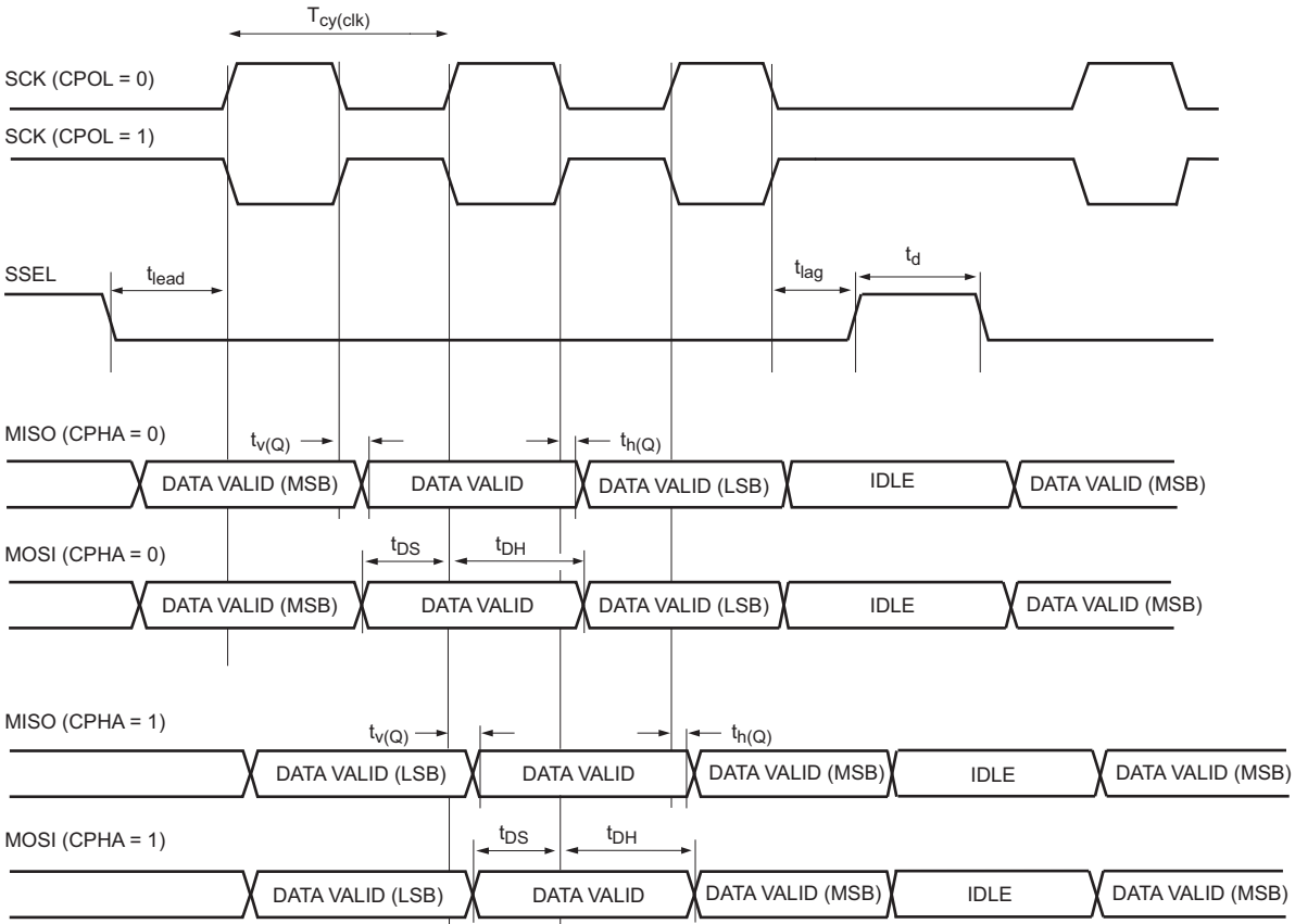
Fig 31. SSP in SPI mode and SPI slave timing
