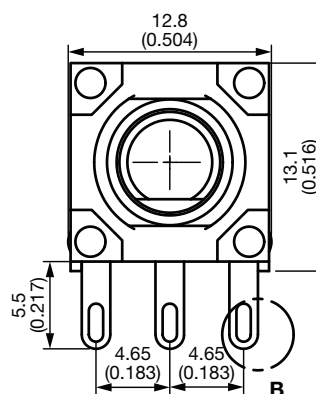
Shaft view at middle travel
