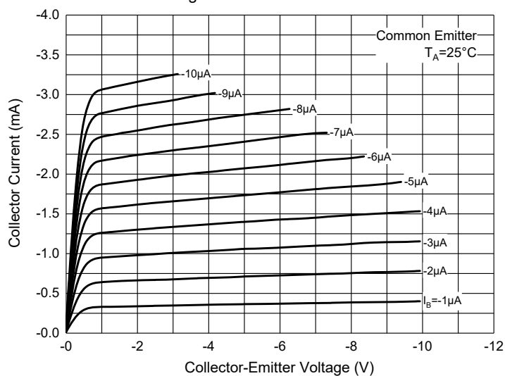
Fig. 7 - Static Characteristics
