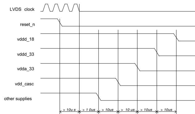
Figure 15. Power-down Sequence
