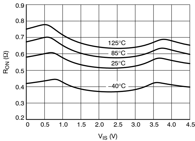
Figure 13. ON Resistance vs. Switch Voltage @ V_{CC} = 4.5\text{ V}
