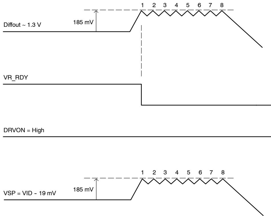
Figure 29. OVP Shutdown
