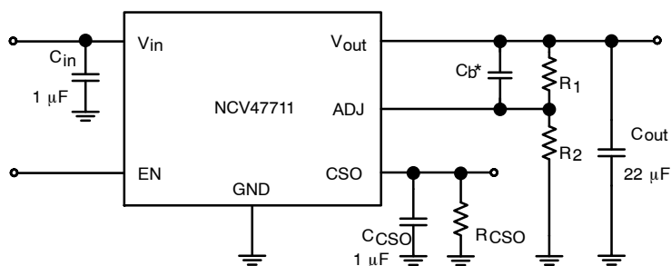
Figure 1. Application Schematic
