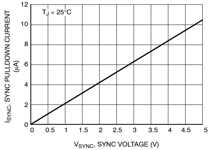
Figure 4. Sync Pulldown Current vs. Sync Voltage
