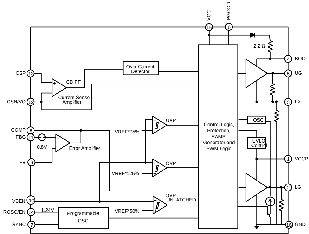
Figure 1. NCP81147 BLOCK DIAGRAM
