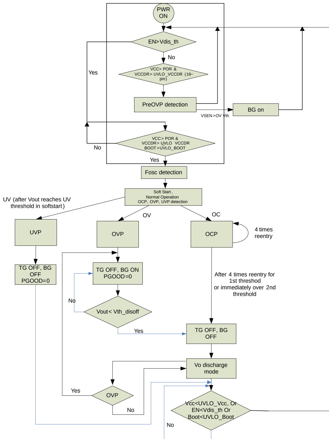
Figure 8. State Diagram
