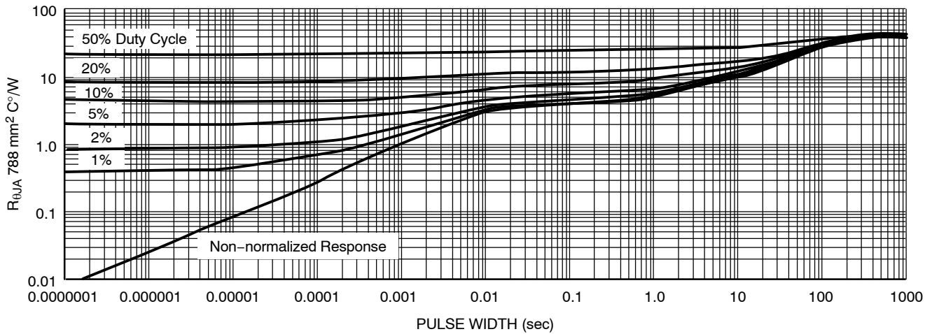
Figure 29. Duty Cycle for 1" Spreaders Boards, D 2 PAK 5-Lead
