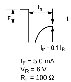
OUTPUT PULSE
