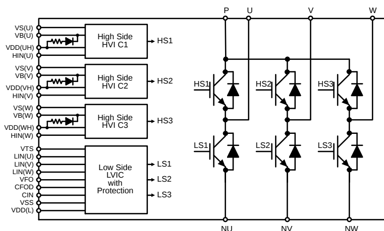
Figure 1. Application Schematic
