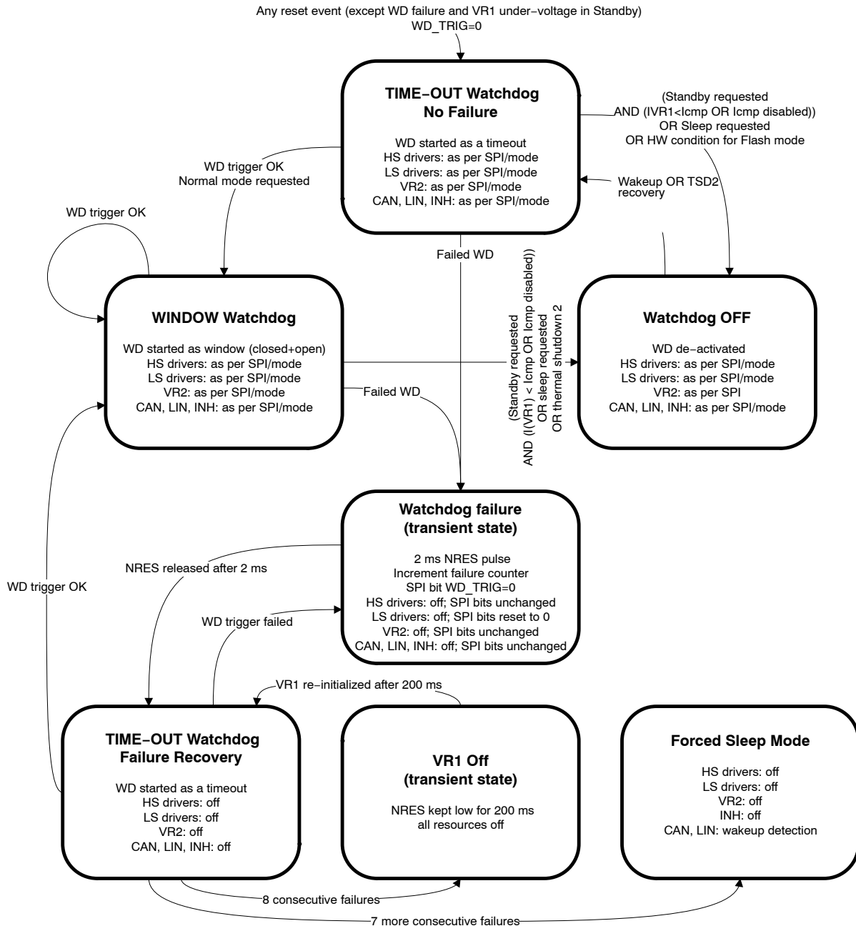
Figure 14. Watchdog Operation
