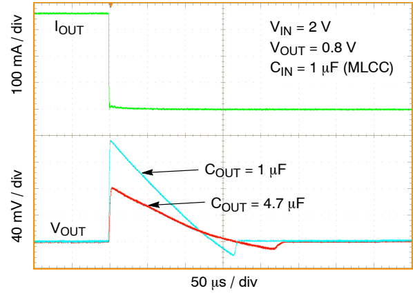
Figure 42. Load Transient Response – Falling Edge, V_{OUT} = 0.8 \text{ V} , I_{OUT} = 1 \text{ mA} to 300 \text{ mA} , C_{OUT} = 1 \mu\text{F} , 4.7 \mu\text{F}
