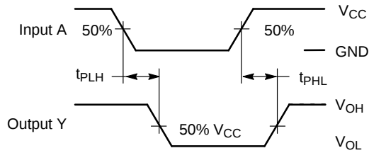
Figure 5. Switching Waveform
