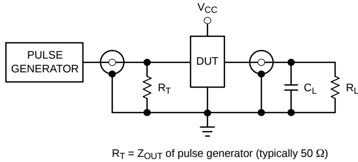
Figure 6. Test Circuit
