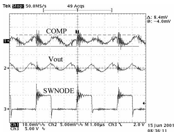
Figure 26. At Full-Load (28 A) the Peak-to-Peak Voltage Ripple on the COMP Pin Should Be Less than 20 mV for a Well-Tuned/Stable Controller. Higher COMP Voltage Ripple Will Contribute to Output Voltage Jitter.
