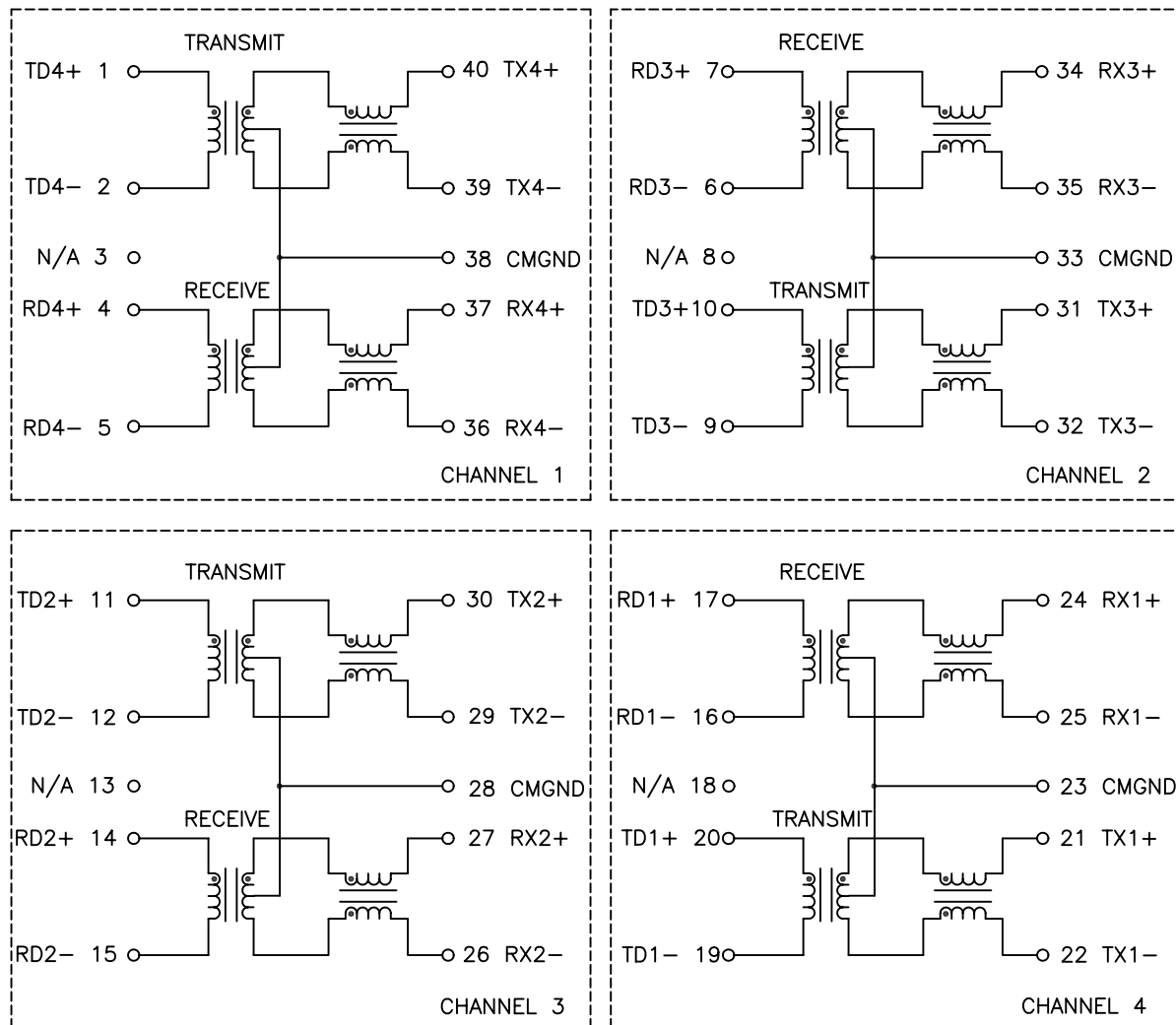
SCHEMATIC
