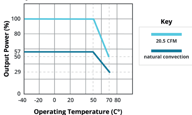
TEMPERATURE DERATING CURVE VMS-350C-24, VMS-350C-27, VMS-350C-36, VMS-350C-48 (full load 350W with 20.5 CFM)
