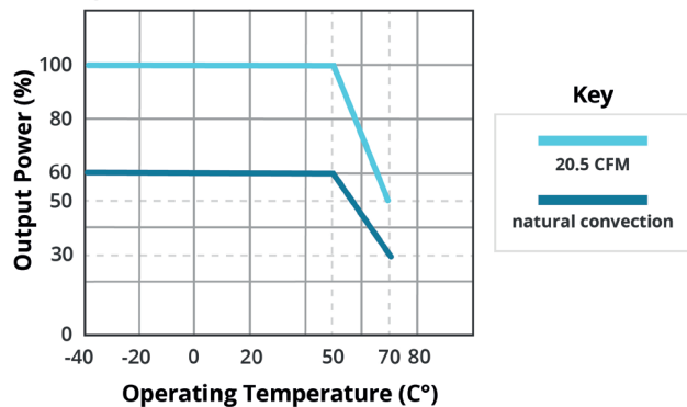
TEMPERATURE DERATING CURVE VMS-350C-12 (full load 300W with 20.5 CFM)
