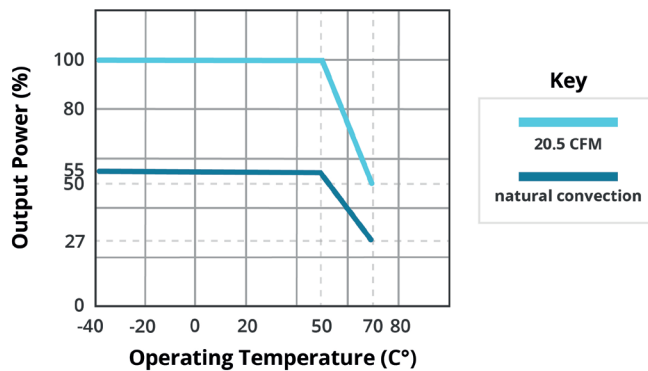
TEMPERATURE DERATING CURVE VMS-350C-15 (full load 325W with 20.5 CFM)
