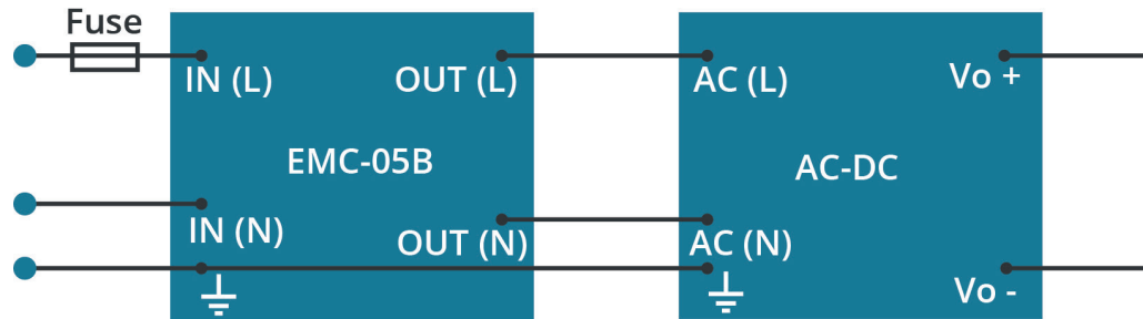
Figure 2 Application Circuit
