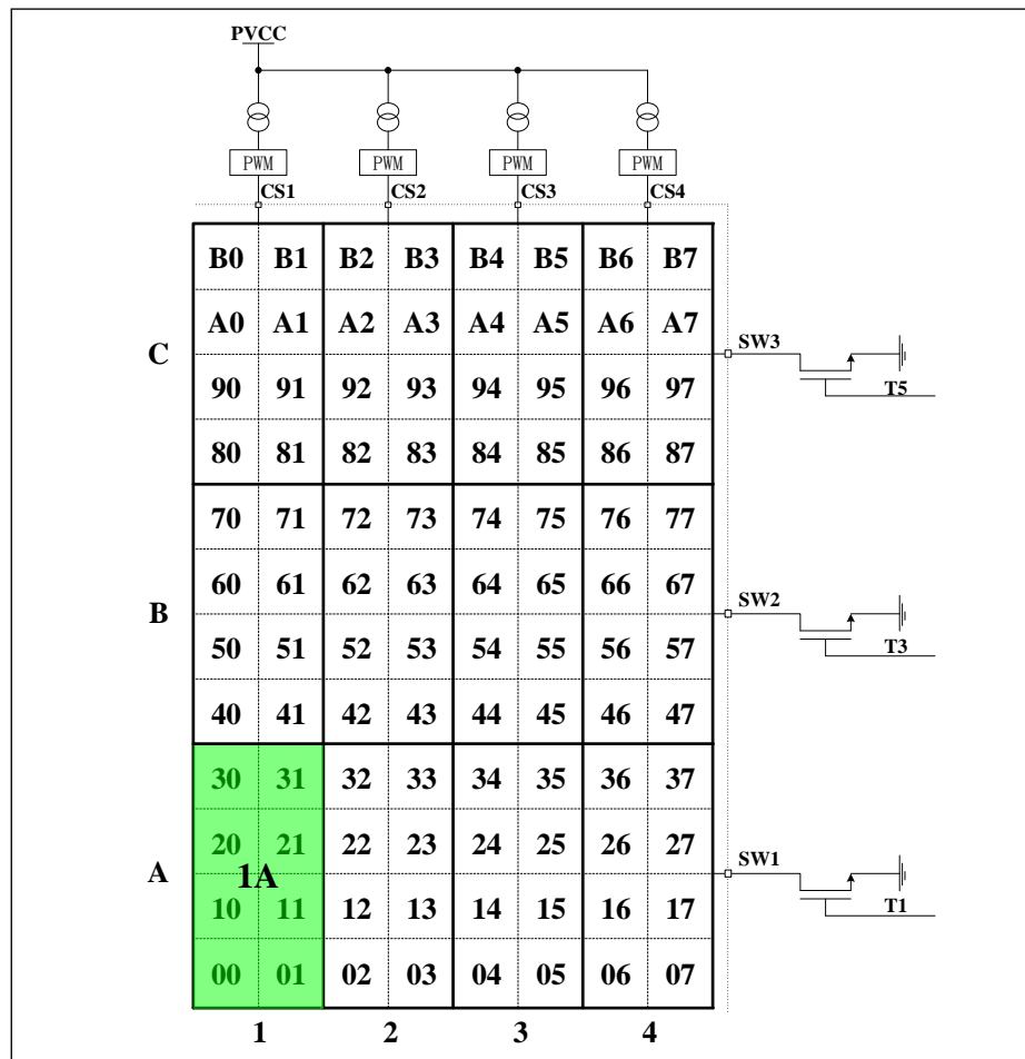
Figure 12 PWM Register
