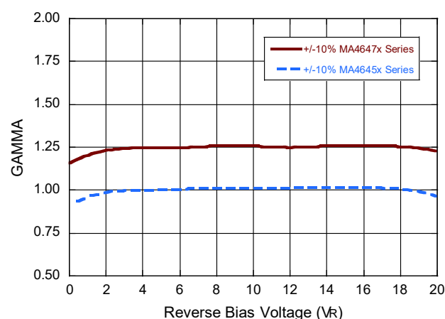
Gamma vs. Reverse Bias Voltage
