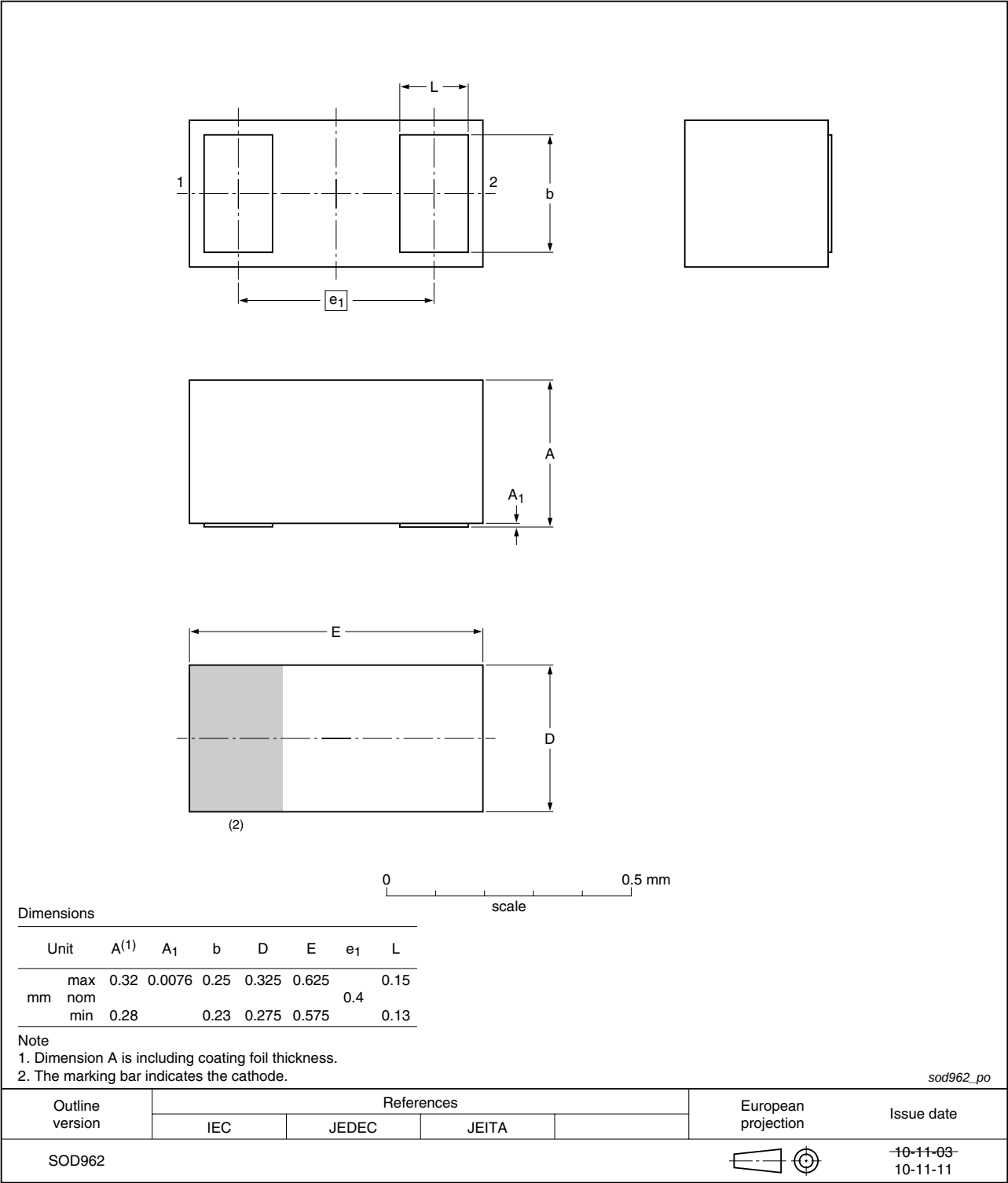
Fig 11. Package outline PESD5V0V1BSF (SOD962)
