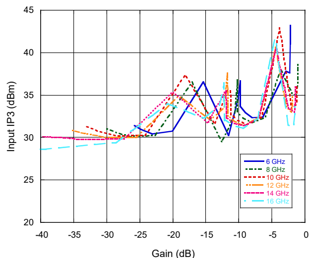
Input IP3 vs. Attenuation, SCL P_{IN} = 12 dBm
