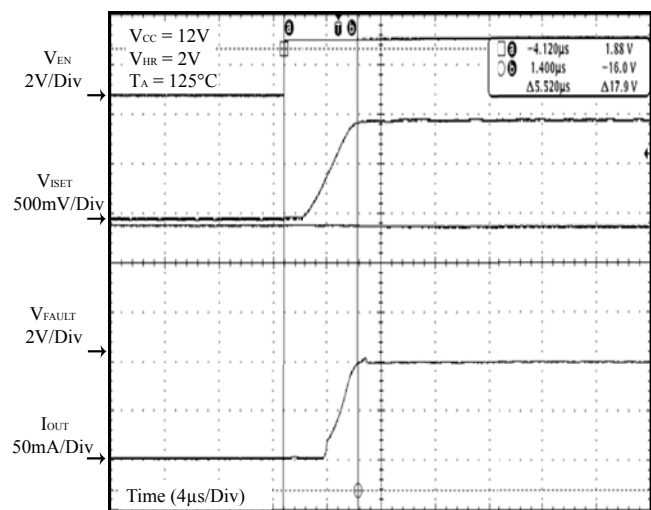
Figure 28 EN On
