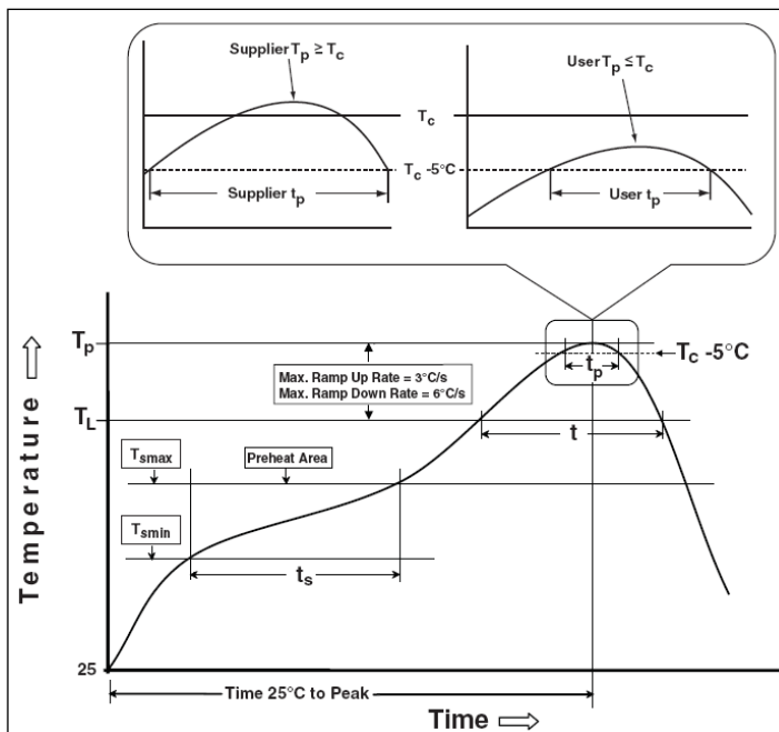
Figure 36 Classification Profile
