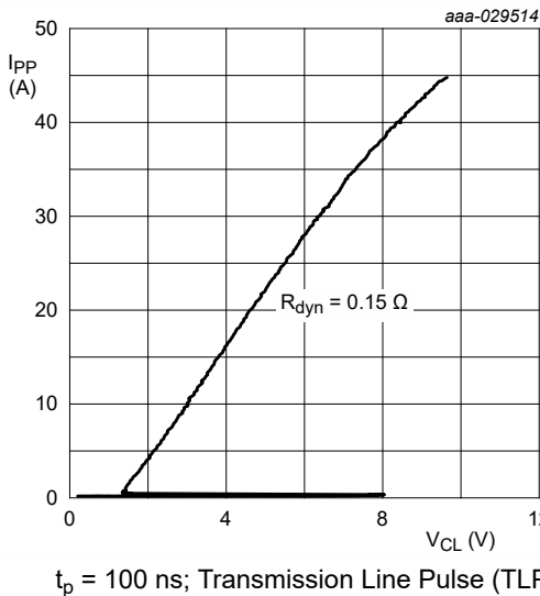
Fig. 5. Positive clamping voltage (TLP); typical values
