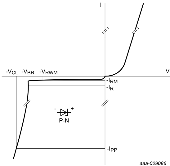
Fig. 3. V-I characteristics
