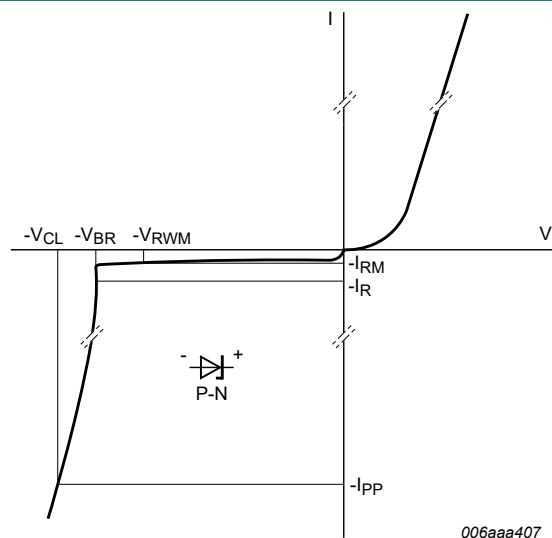
Fig. 8. V-I characteristics for a unidirectional ESD protection diode
