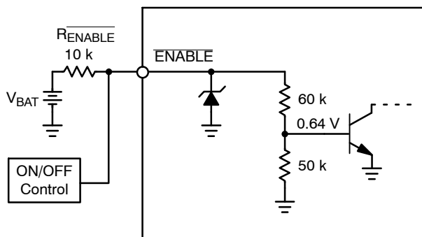
Figure 7. Using the ENABLE pin with V BAT
