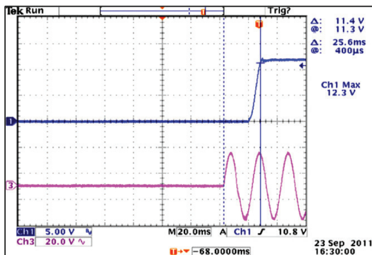
12V OUT, FULL LOAD, 264VAC
