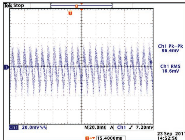
12V OUT, FULL LOAD, 230VAC, 60HZ
