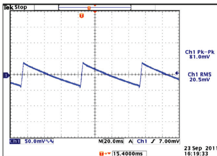
12V OUT, NO LOAD, 230VAC, 60HZ
