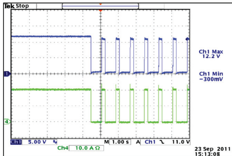
12V OUT, 90VAC
