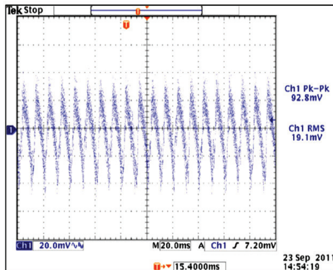
12V OUT, FULL LOAD, 115VAC, 60HZ
