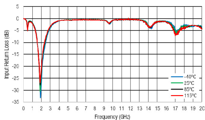
Figure 54. Input Return Loss (dB) vs Frequency (GHz)
