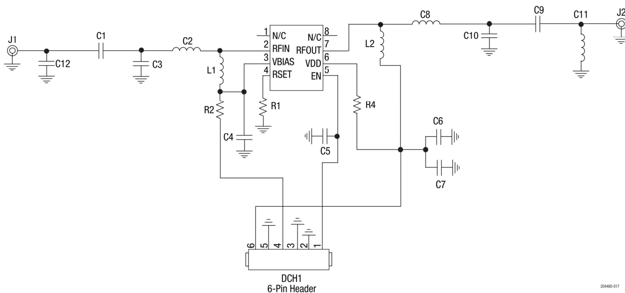
Figure 59. SKY67183-396LF Evaluation Board Schematic
