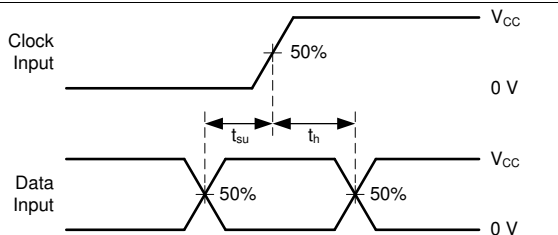
Figure 7. Voltage Waveforms, Setup and Hold Times
