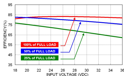
EDL02-24S05 Efficiency vs. Input Voltage
