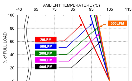
EDL02-24S05 Derating Curve
