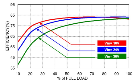
EDL02-24S05 Efficiency vs. Output Load
