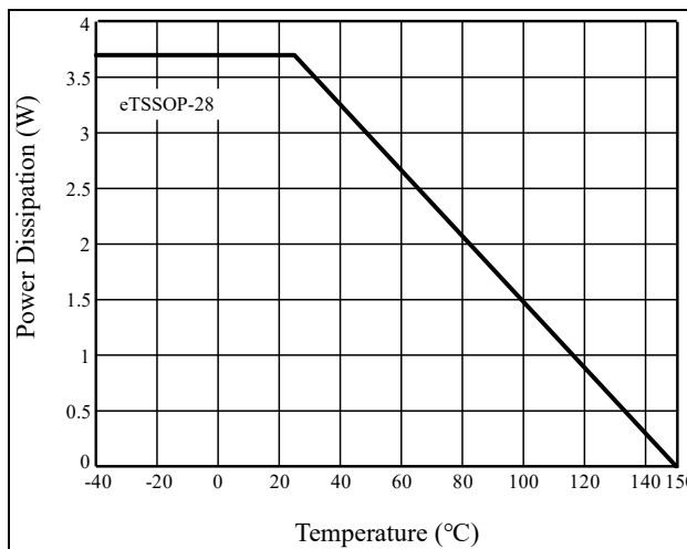
Figure 8 Dissipation Curve
