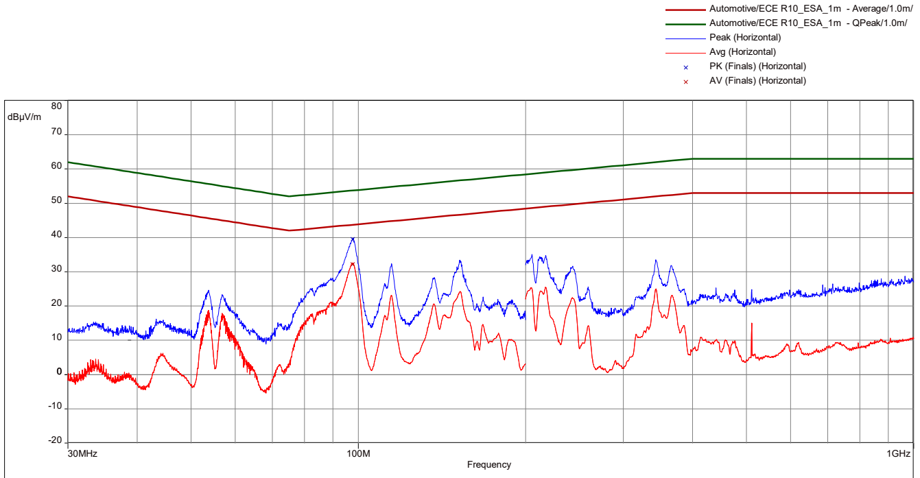
Fig. 10 12RCM60-24: Typ. radiated disturbances in 1 m distance ( V_i = 13.5\text{ V} , I_{i\text{ nom}} , resistive load, peak & average)
