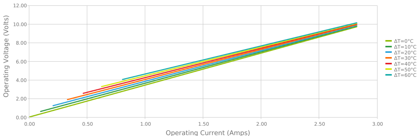
Current vs Voltage (I vs V) T_{\text{hot}} = 85^\circ\text{C}
