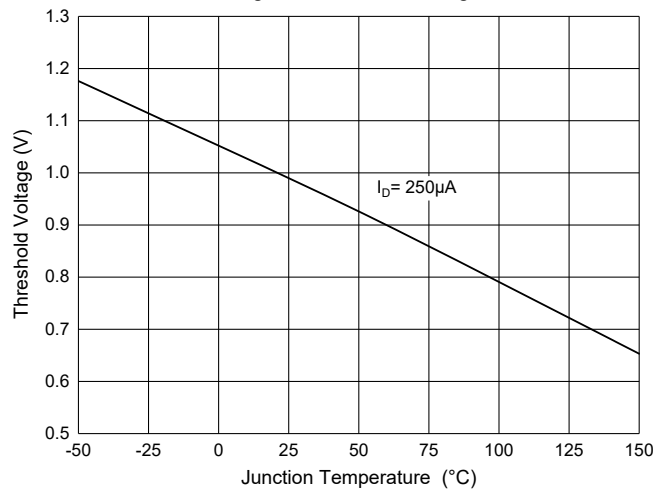
Fig. 6 - Threshold Voltage
