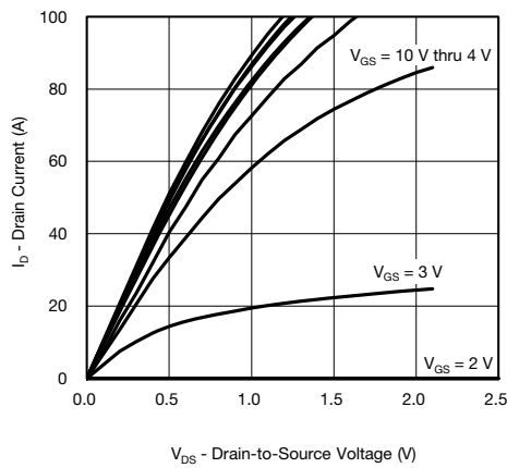
Output Characteristics
