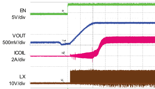
Fig. 15 - Load Step Undershoot Response I_{OUT} = 0\text{ A} to 3\text{ A} , Time = 1\text{ ms/div}
