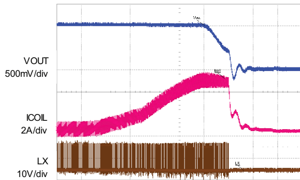
Fig. 16 - Over Current Protection, I_{VALLEY} = 4\text{ A} , Time = 100\text{ }\mu\text{s/div}
