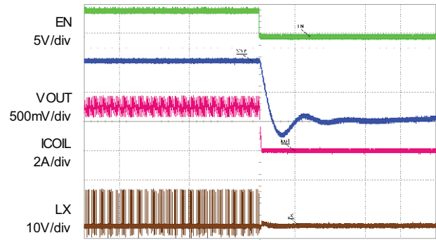
Fig. 17 - Shut-Down, I_{OUT} = 3\text{ A} , Time = 50\text{ }\mu\text{s/div}
