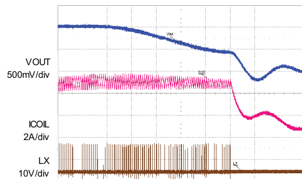
Fig. 18 - Over Current Protection, I_{VALLEY} = 4\text{ A} , Time = 20\text{ }\mu\text{s/div}
