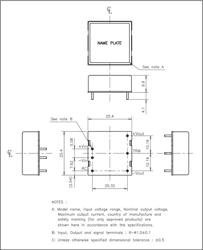
Outline Drawing CCG30-S (Single Output)
