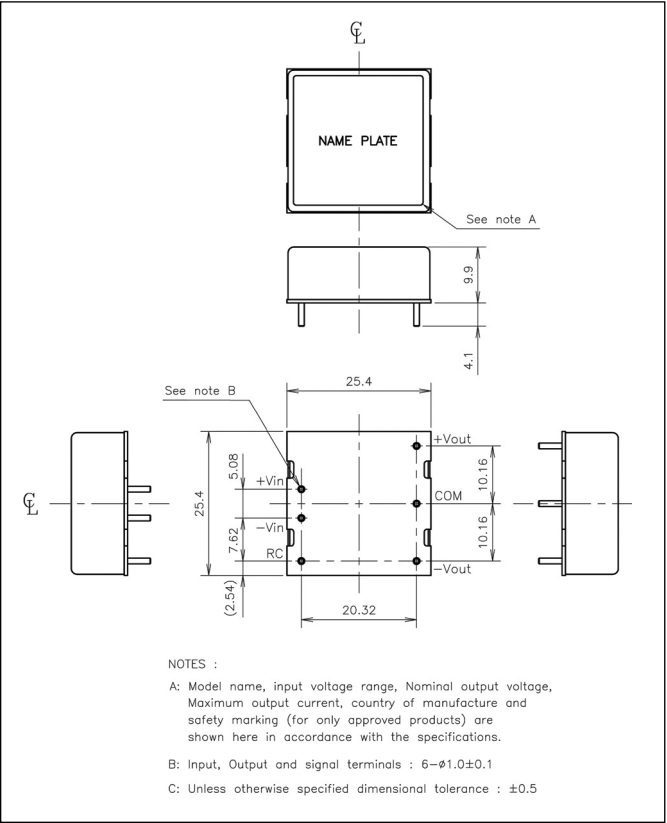
Outline Drawing CCG30-D (Dual Output)
