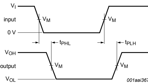
Fig. 13. The data input (nAn, nBn) to output (nBn, nAn) propagation delay times
