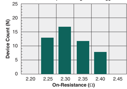
Typical On-Resistance Distribution (N=50, I_F=5\text{mA} , I_L=350\text{mA}_{DC} )
