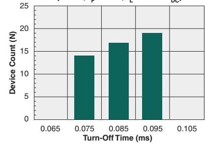
Typical Turn-Off Time (N=50, I_F=5\text{mA} , I_L=350\text{mA}_{DC} )
