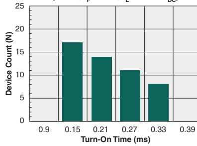
Typical Turn-On Time (N=50, I_F=5\text{mA} , I_L=350\text{mA}_{DC} )
