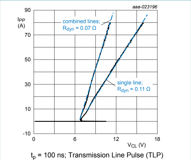
Fig. 7. Dynamic resistance with positive clamping voltage; typical values
