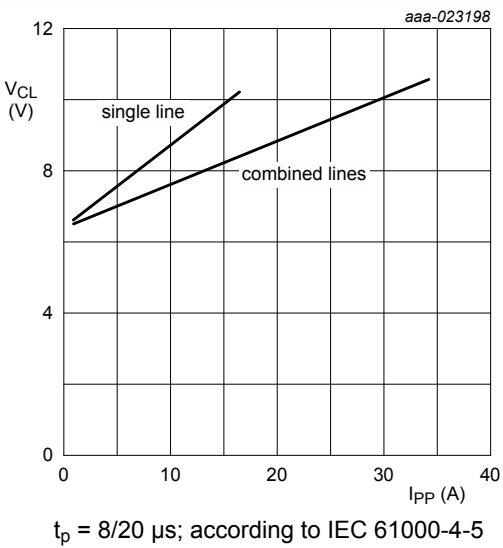
Fig. 9. Dynamic resistance with positive clamping voltage; typical values
