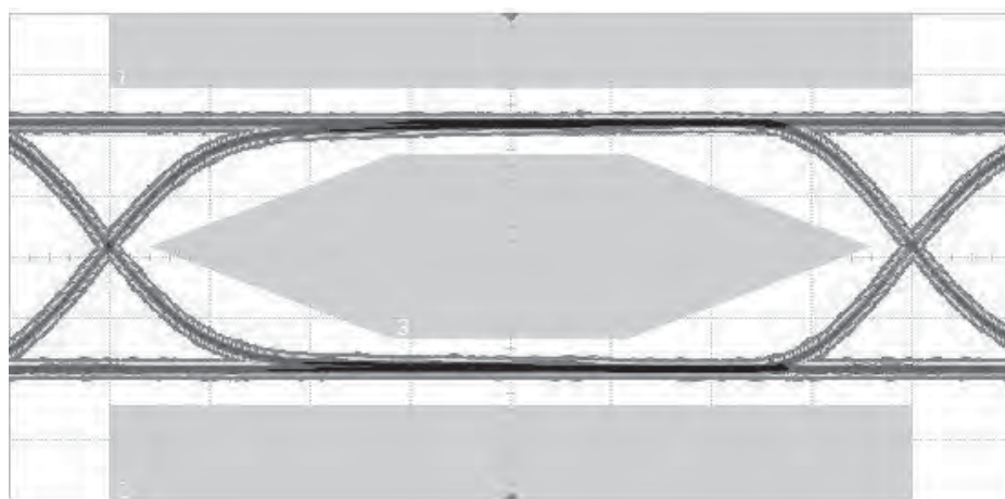
Fig 7. USB 2.0 eye diagram with IP4369CX4
