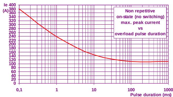
CURRENT OVERLOAD CHARACTERISTIC
