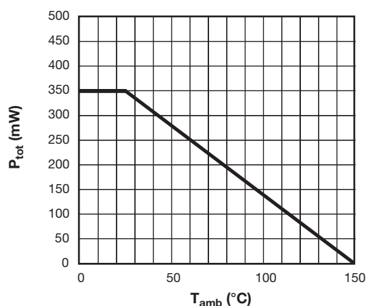
Fig. 1 - P_{tot} - Admissible Power Dissipation vs. Ambient Temperature
