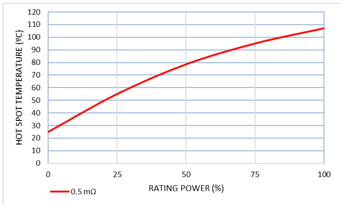
Rated Power vs. Surface Temperature – HCS1206
