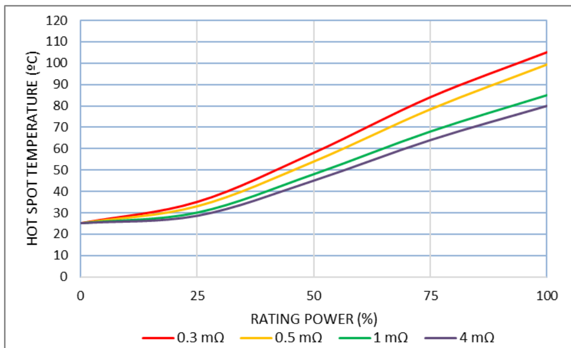
Rated Power vs. Surface Temperature – HCS3920
