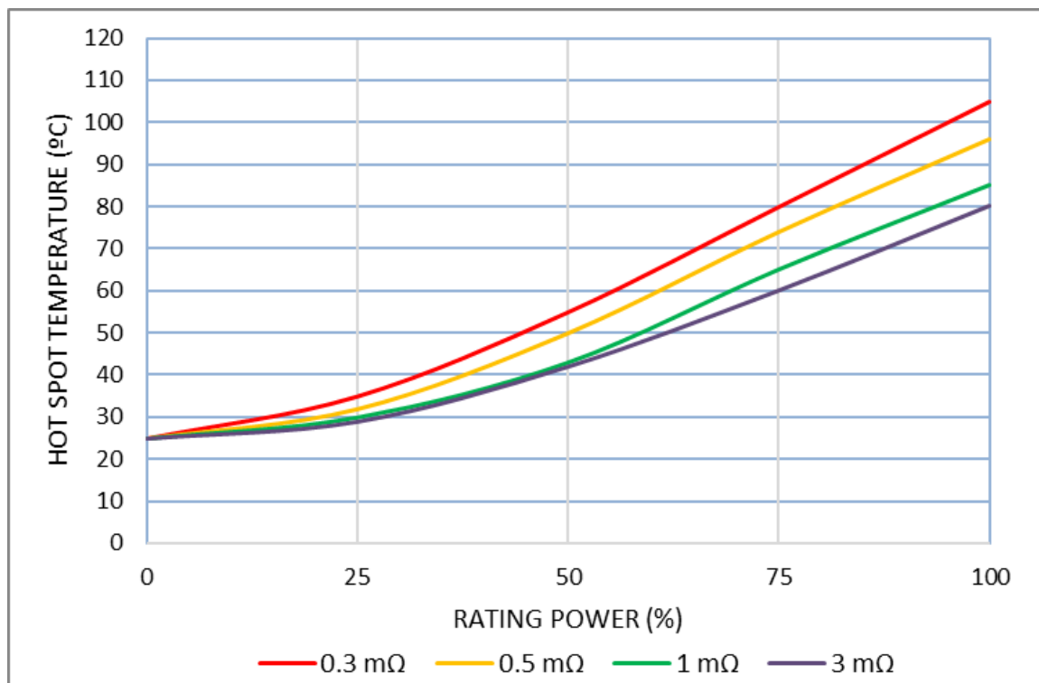
Rated Power vs. Surface Temperature – HCS2512
