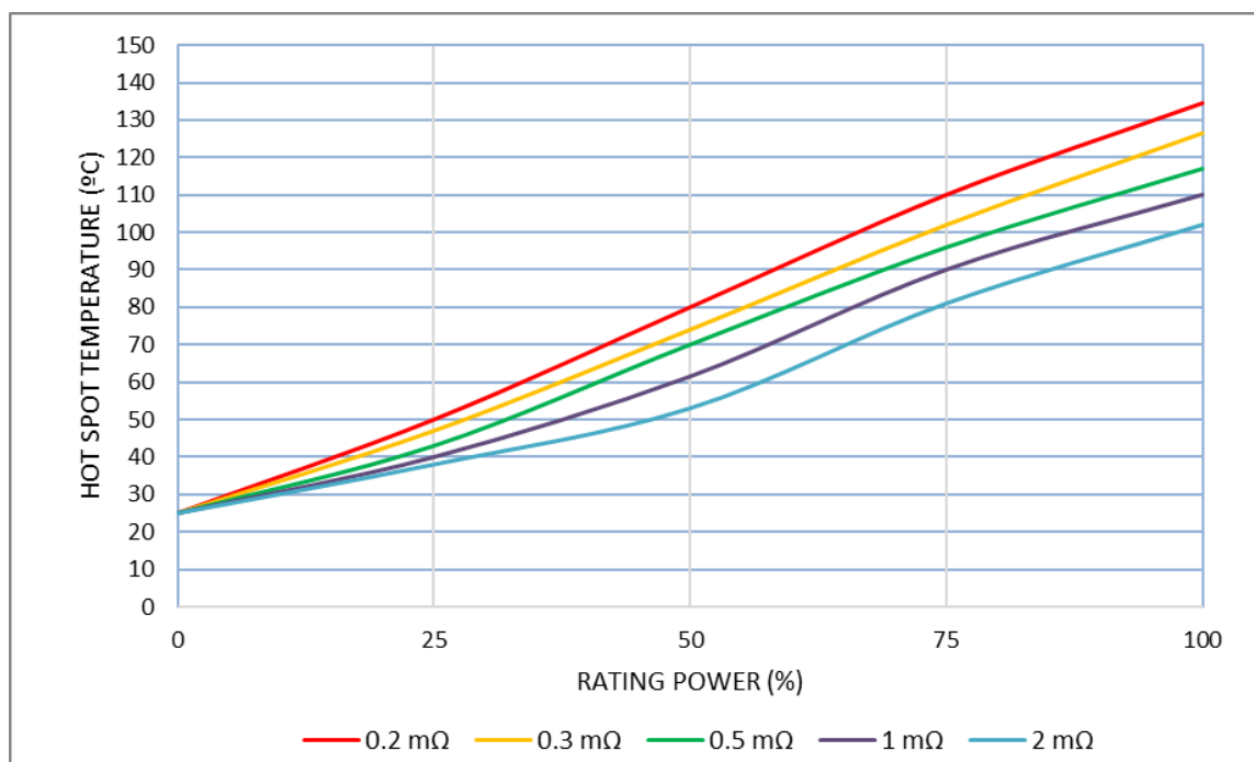
Rated Power vs. Surface Temperature – HCS5930
